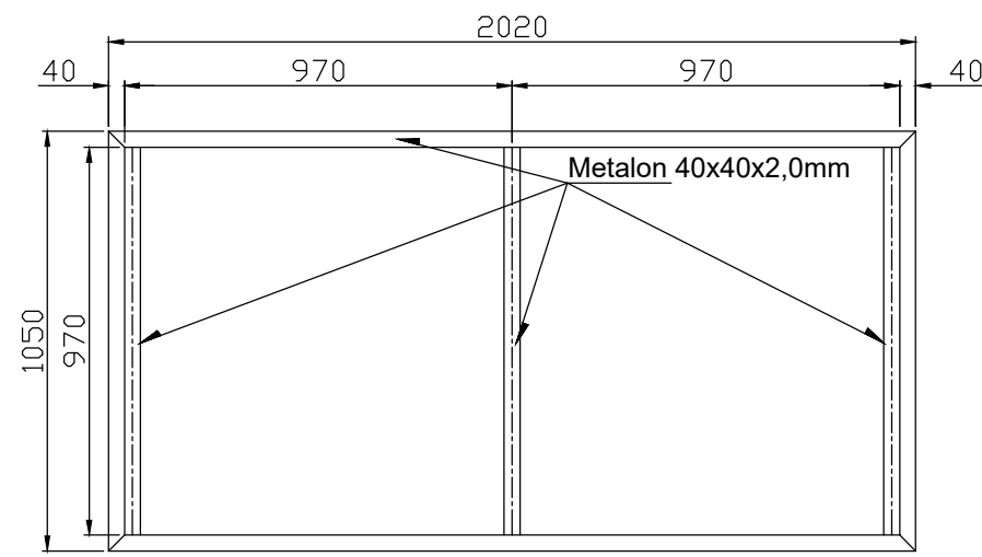
VISTA FRONTAL
